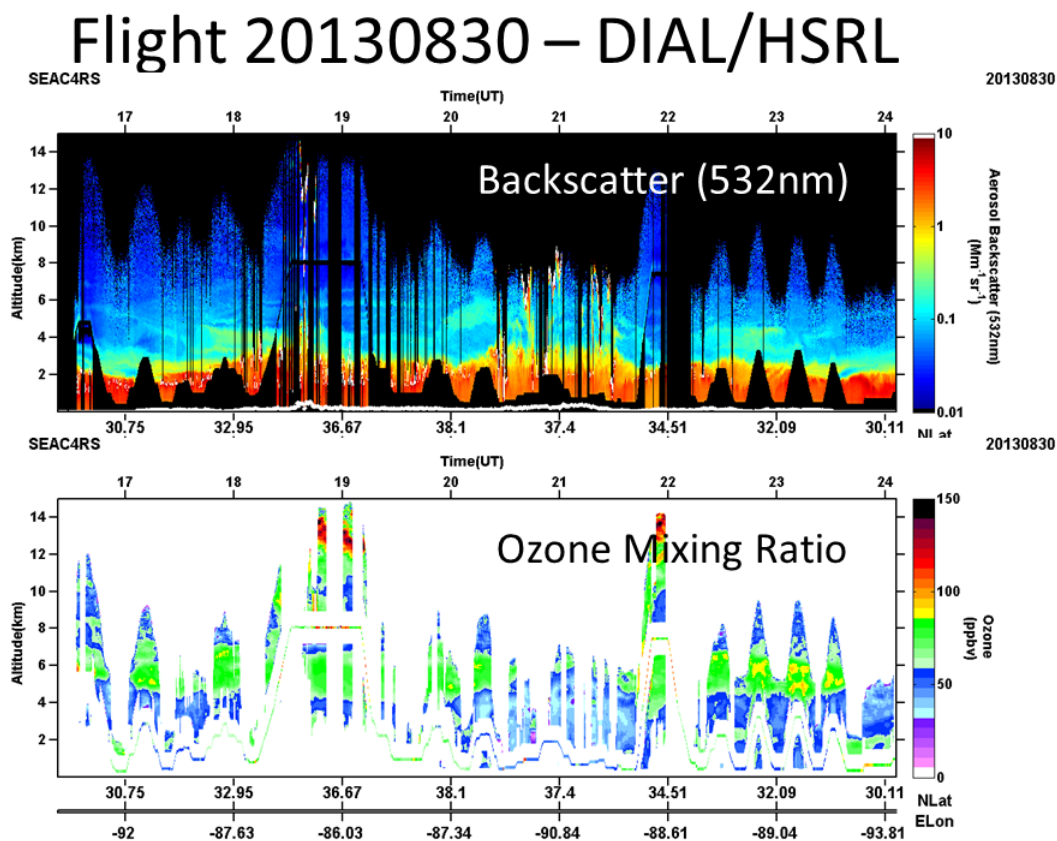
Figure 2. DIAL/HSRL aerosol backscatter and ozone mixing ratio curtains along the August 30, 2013 DC-8 flight track.
