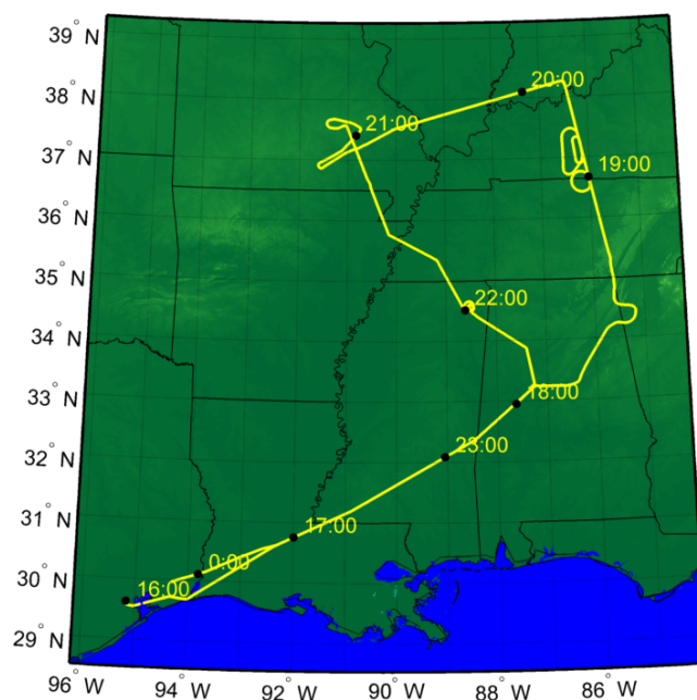
Figure 1. DC-8 flight track for August 30, 2013.
