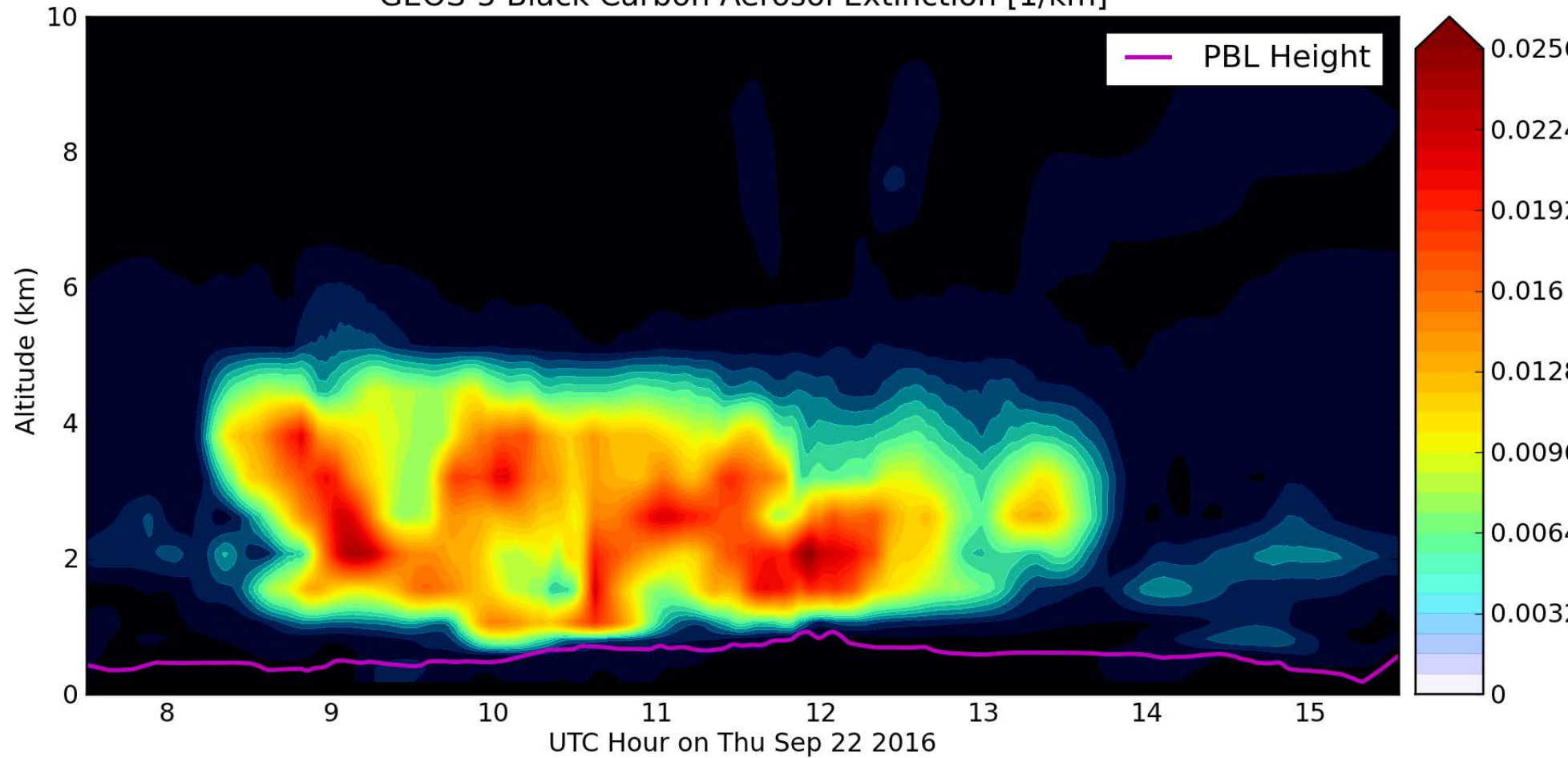
GEOS-5 Black Carbon Aerosol Extinction [1/km]
