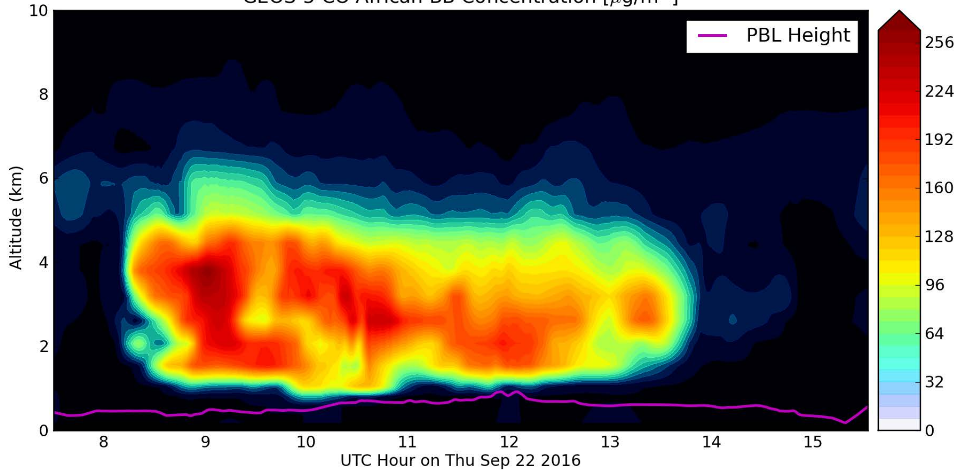
GEOS-5 CO African BB Concentration [ \mu\text{g}/\text{m}^3 ]
