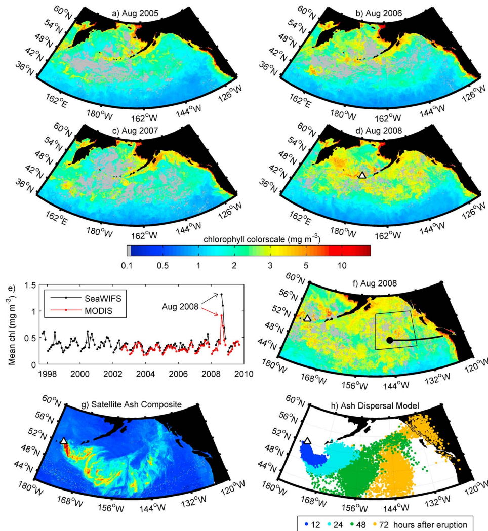
Figure 1. (a–d) North Pacific MODIS monthly-averaged surface chlorophyll in August 2005, 2006, 2007, 2008. (e) Time-series of monthly mean chlorophyll averaged over box shown in Figure 1f. (f) Zoom on subarctic NE Pacific MODIS August 2008 chlorophyll, same spatial grid as Figures 1g and 1h. Box shows area of time series averaging. Line from coast shows mid-August cruise track. Point at end of line shows Station P. White triangles show Kasatochi volcano. (g) Composite of most intense satellite detections of airborne ash from the Kasatochi eruption. (h) Particle locations at 0–10,000 m altitude from ash dispersal model at 12, 24, 48, and 72 hours after the start of the Kasatochi eruption.
