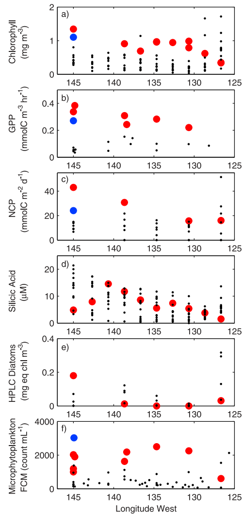
Figure 3. Red circles show measurements along a cruise transect from 15 August (coastal at 125°W) to 21 August 2008 (Station P at 145°W). Blue circles show measurements at Station P on 31 August. Black dots show measurements from other years. For (a) chlorophyll and (d) silicic acid, black dots show Aug or Sep measurements in 1988–2004 [Peña and Varela, 2007]. For (b) GPP and (f) FCM data, black dots show June and August 2007, and June 2008. For (c) NCP, black dots show June and August 2007–2009, excepting August 2008. For (e) HPLC data, black dots show September 2006, June and August 2007, and June 2008.
