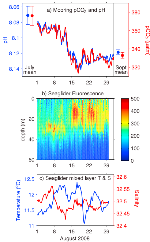
Figure 2. (a) Aqueous pCO 2 (red) and pH (blue) measured at the surface from a mooring at Station P. pH scale is reversed. Means and standard deviations for July and September 2008 shown. (b) Raw chlorophyll fluorescence signal measured by a Seaglider within 35 km of Station P. (c) Seaglider temperature and salinity averaged over upper 20 m.
